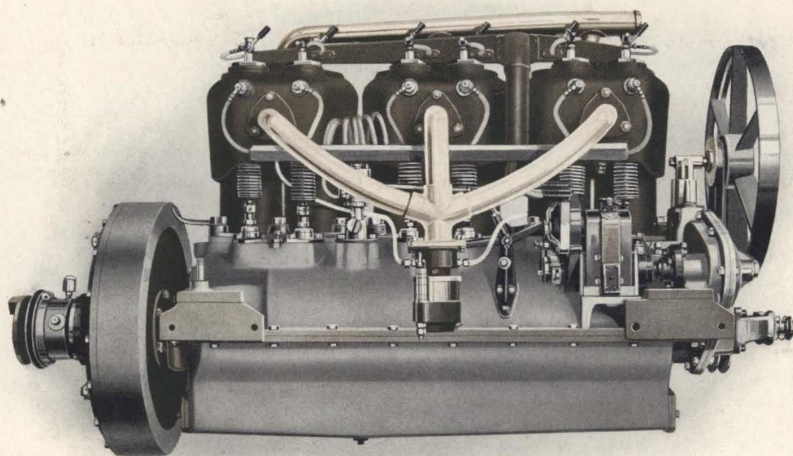
Inlet Side of "Six-Forty" Motor
