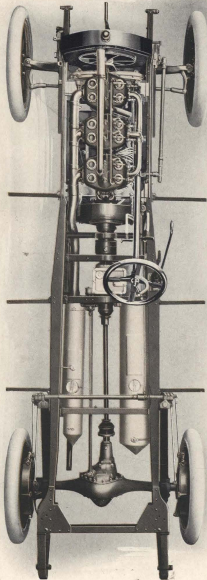
Thomas "Six-Forty," Touring Car Chassis
